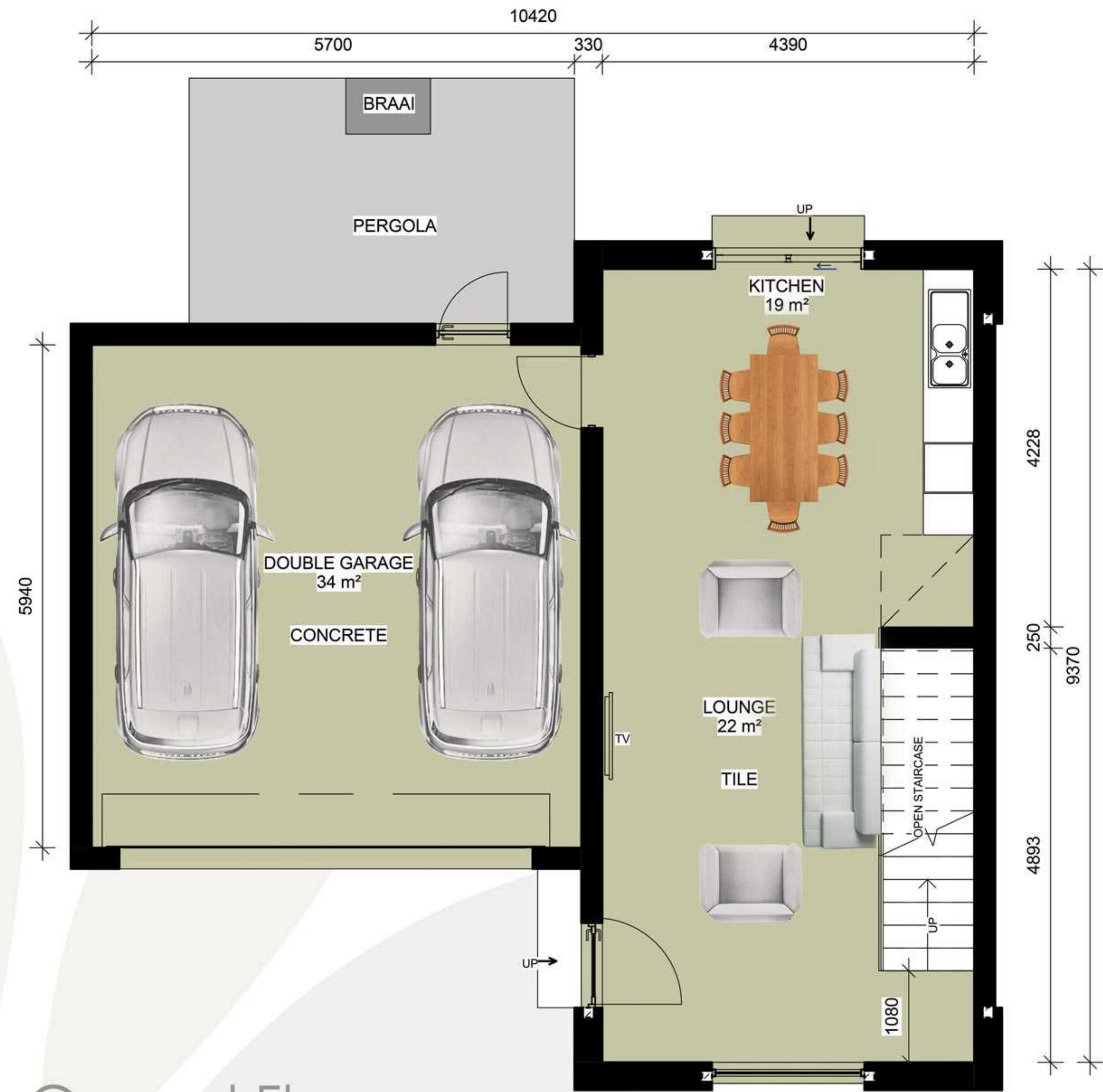
Ground Floor
